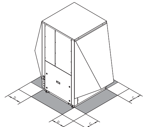
Outdoor installation
